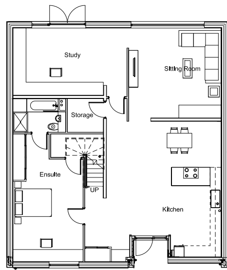
1 Existing Ground Floor Plan 203 1:100@A3
