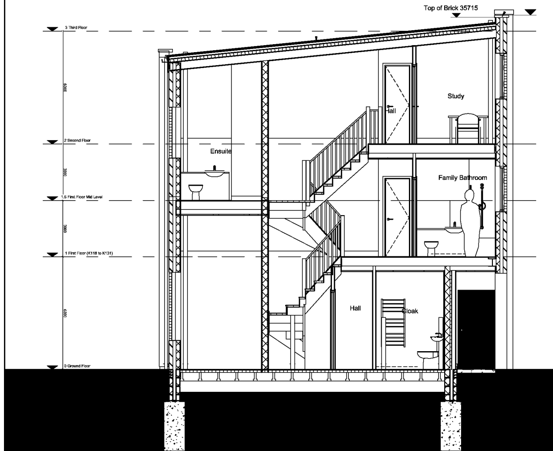
1 Section As Proposed 206 1:100@A3
